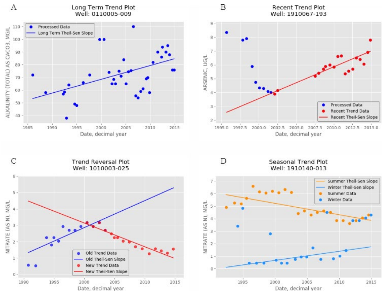
Figure 4-2. Examples of (A) long-term, (B) recent, (C) reversing, and (D) seasonal trends (Modified from Figure 1 [Dupuy et al., 2019]).
