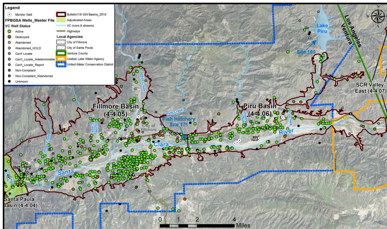
Figure 1-1: Fillmore and Piru basins area map showing FPGSA's well inventory displayed by Ventura County well status and select monitor wells.
