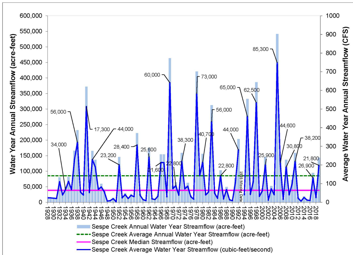
Figure 2-8: Sespe Creek historical annual streamflow (streamflow data from USGS and VCWPD). Labeled values shown are peak flows (CFS) for select water years.
