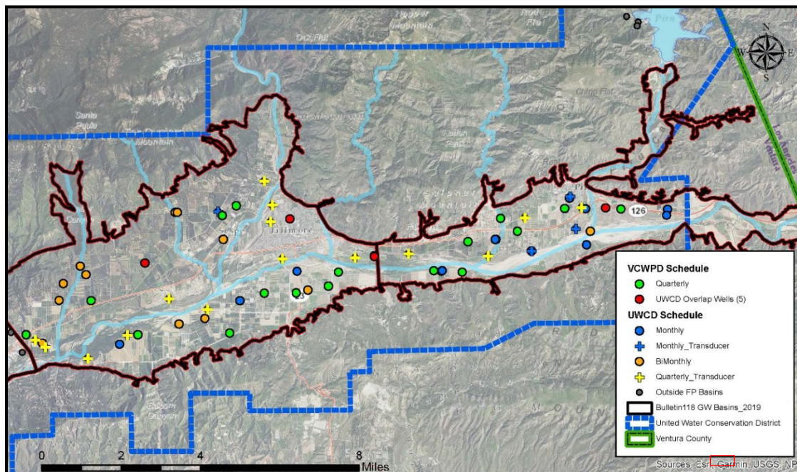
Figure 3-2: UWCD and VCWPD active status groundwater level measurement well sites and schedules.
